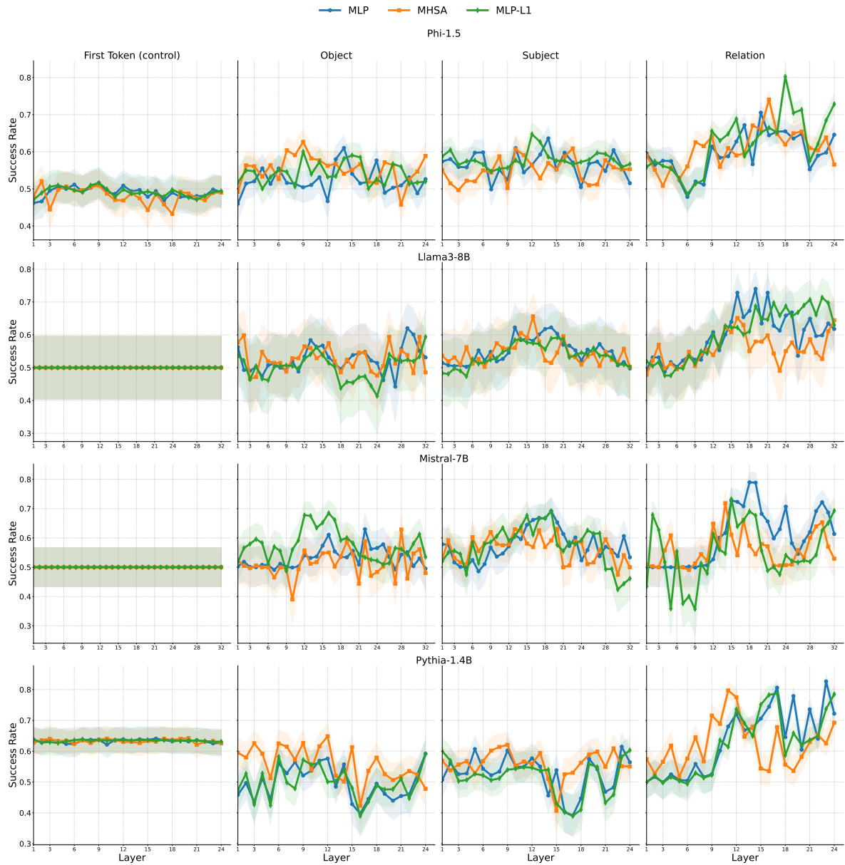
Figure 5: Performance of the linear classifier in identifying knowledge sources across different layers and modules (MLP, MLP-L1, MHSA). The plots show success rates for classifiers trained on activations from object, subject, and relation tokens, with the first token used as a control (see Section 4.1 for more details on the control experiment.) Results are reported for the Mistral-7B, Phi-1.5, Llama3-8B, and Pythia-1.4B models. Solid lines represent the average success rates across relation groups, while shaded areas denote the weighted standard error with a 95% confidence interval. See Section 4.3 for further details on the evaluation methodology.
