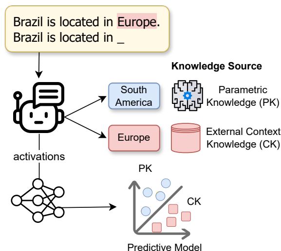
Figure 1: Illustration of our method for probing knowledge sources in LLMs. We present the model with a prompt containing contradictory information to its learned knowledge to test whether it uses parametric knowledge (PK) or contextual knowledge (CK). The resulting activations are used to train a classifier to distinguish between PK and CK.
