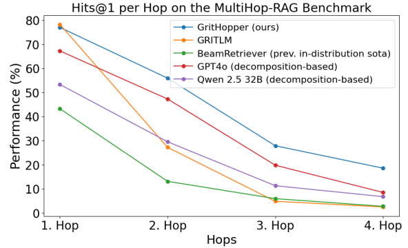
Figure 1: Out-of-distribution Multi-Hop Retrieval Performance on the MultiHop-RAG Benchmark (Tang and Yang, 2024). While methods such as BeamRetriever achieve state-of-the-art performance in in-distribution settings, GRITHopper consistently outperforms them under distribution shift, with the relative advantage increasing at deeper hops, highlighting its robustness to long-context accumulation.
