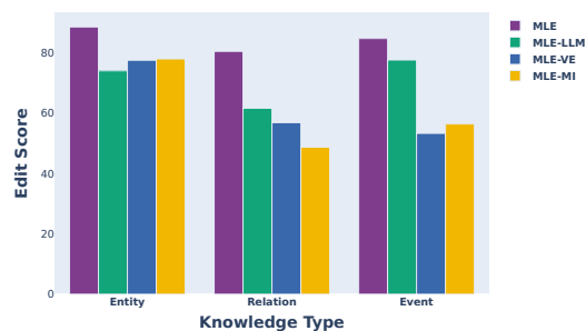
Figure 6: The result of MLE edits different components of BLIP2-OPT 6.7B.
