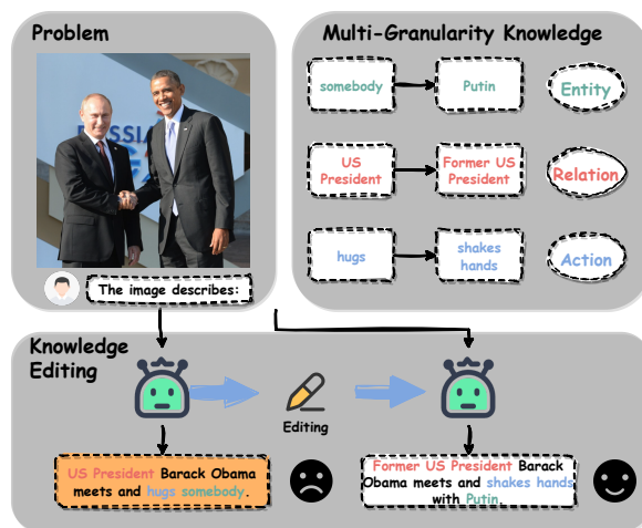
Figure 1: Overview of Multi-Granularity Knowledge Editing. After editing multi-granularity knowledge (knowledge that includes three distinct forms: entity , relation , action ) in the multimodal large language model, it can solve the problem correctly.
