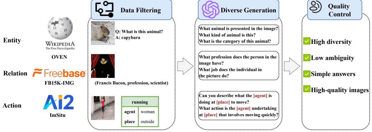
Figure 7: Data Annotation Process Flowchart. First, raw samples of Entities, Relations, and Actions are filtered from Oven, FB15K-IMG, and ImSitu based on predefined rules. Next, the raw data is transformed into QA-form datasets using ChatGPT, incorporating diverse variations. Finally, high-quality data is manually curated to construct the M2Edit dataset.
