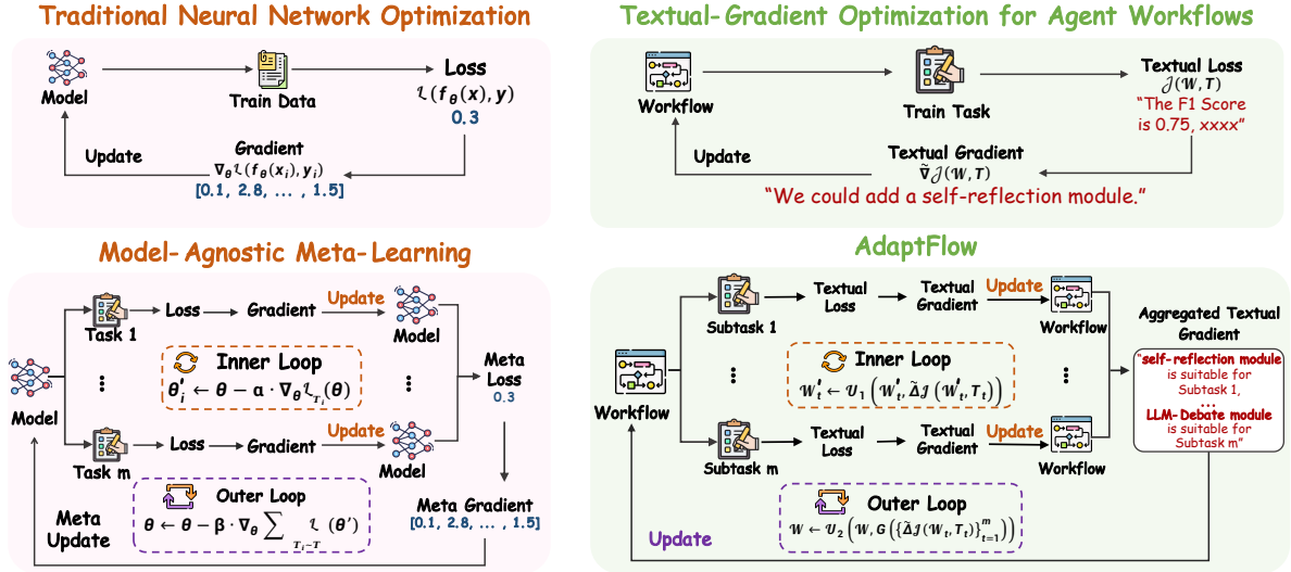
Figure 1: An analogy between Neural Network Optimization and Workflow Optimization, as well as between MAML and AdaptFlow.
