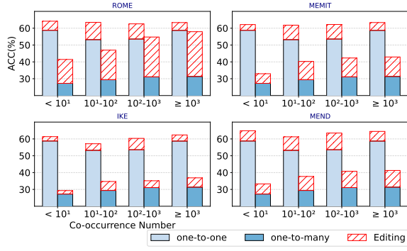
(a) BioGPT
