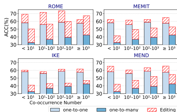
Figure 6: The knowledge probing performance of BioMedLM on both one-to-one knowledge and one-to-many knowledge before and after editing.
