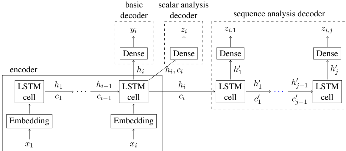
Figure 3: Network architecture of the model. The basic end-to-end model consists of the encoder and the basic decoder. The analysis model fixes the weights for the encoder and uses the scalar (if z_i is a scalar) or sequence analysis decoder (if z_i is a sequence).
