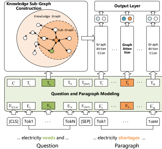
Figure 1: Framework of our SKG model.
