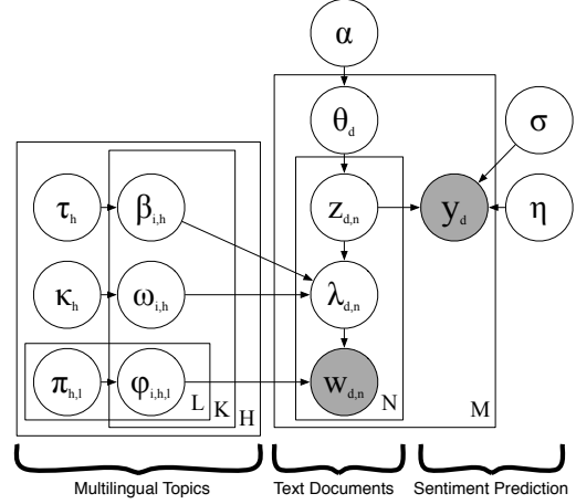
Figure 1: Graphical model representing MLSLDA. Shaded nodes represent observations, plates denote replication, and lines show probabilistic dependencies.
