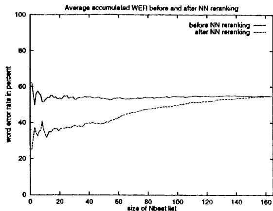
Figure 2: Cumulative average WER before and after reranking for an example utterance
