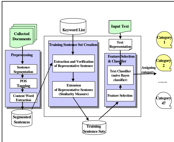
Figure 1: Architecture for the proposed system
