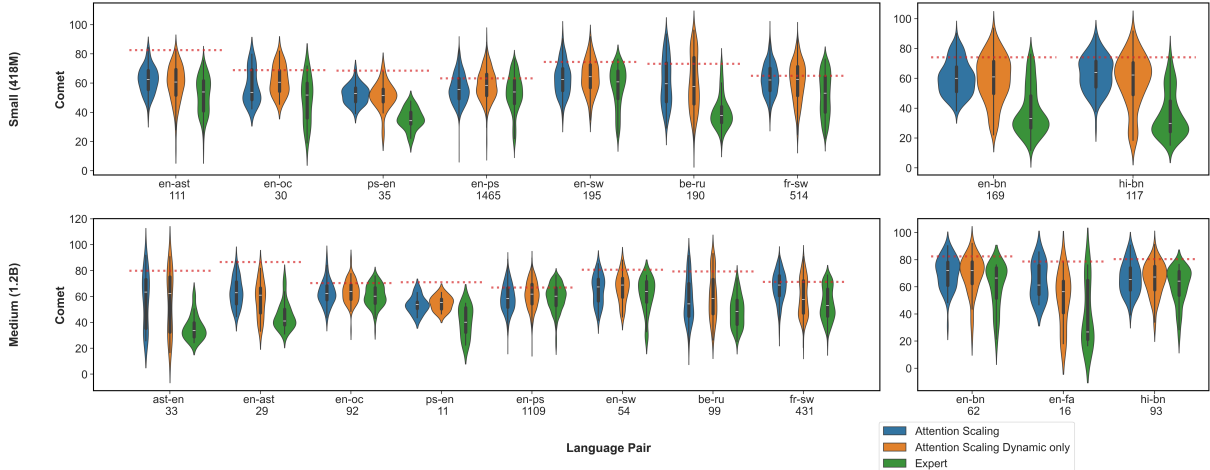
Figure 1: COMET score distributions for hallucinations using the EXPERT and ATTENTION SCALING amateurs for all language pairs with 10 or more hallucinations. Results are given for both the 418M and 1.2B parameter models. The red line is the mean COMET of EXPERT non-hallucinations for a given language pair.
