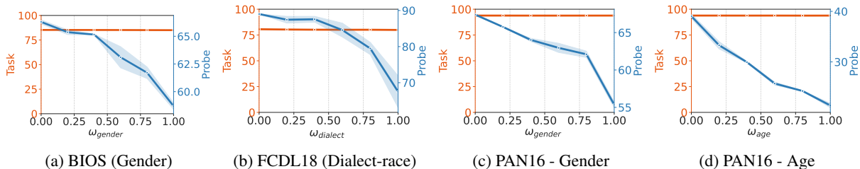
Figure 2: Results of the CONGATER models using BERT-Base when increasing the gating sensitivity \omega from 0 (no effect) to 1 (full effect). Each trained model is evaluated multiple times on the various \omega values adjusted at inference time. The left/right y-axis corresponds to the task performance and attribute probing results, respectively. The results show the continuous reduction in the information presence of the target concept, as \omega increases.
