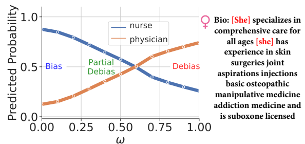
Figure 3: Prediction probabilities of CONGATER when gradually increasing \omega , for a female physician’s biography, incorrectly classified as a nurse in the initial state. The figure illustrates how changing the strength of gender removal affects the model’s decision, providing a higher degree of interpretability through controllability.
