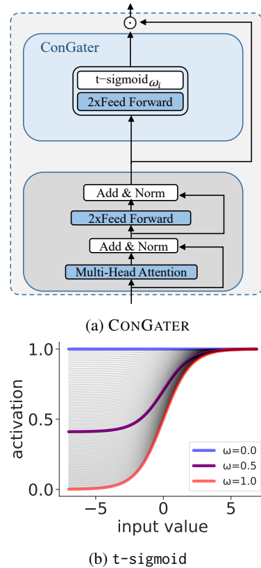
Figure 1: (a) The overall architecture of CONGATER as an adjustable self-gate adapter network. (b) Effect of \omega parameter on t-sigmoid. Increasing \omega results in a transition from the constant function y = 1 (open gate) to the sigmoid function (full functional gate).
