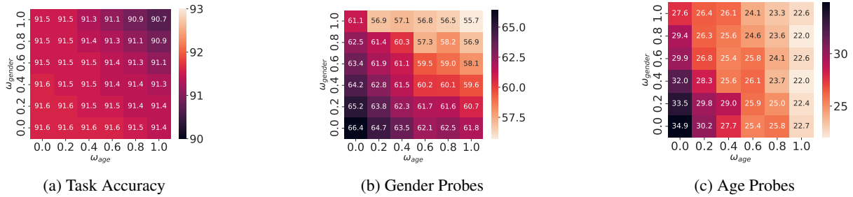
Figure 8: Results of the multi-concept CONGATER on the two attributes of PAN16 task using BERT-Mini, as changing the gender and age \omega simultaneously. (a) Task performance with accuracy (%). (b) Balanced accuracy (%) of gender probes. (c) Balanced accuracy (%) of age probes.
