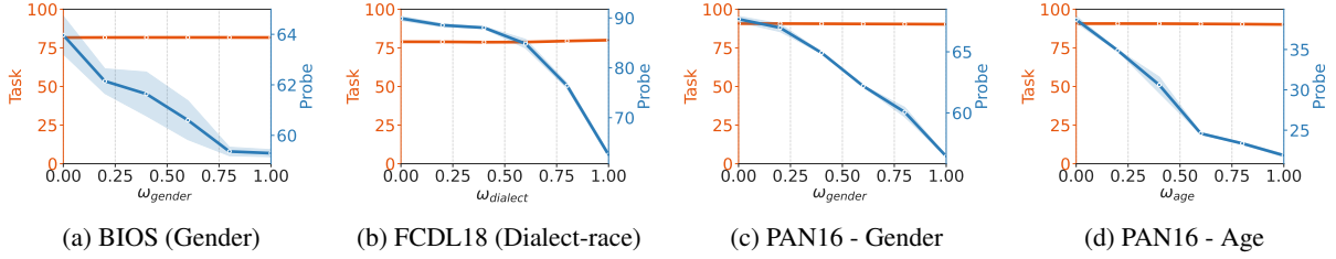
Figure 6: Results of the CONGATER models using BERT-Mini. See Figure 2 for full explanation.
