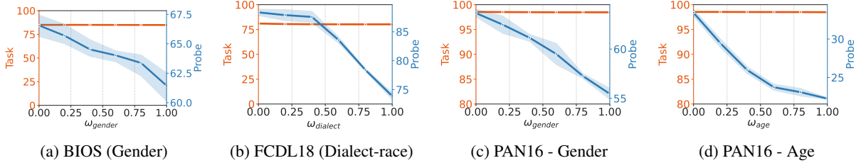
Figure 7: Results of the CONGATER models using RoBERTa-Base. See Figure 2 for full explanation.
