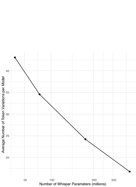
Figure 2: Relation between the numbers of parameters (log scale) of the tiny, base, small and medium models and the detection of Pronunciation Errors Candidates signalled by spelling variants or token additions
