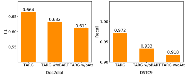
Figure 3: Ablation study for knowledge selection.
