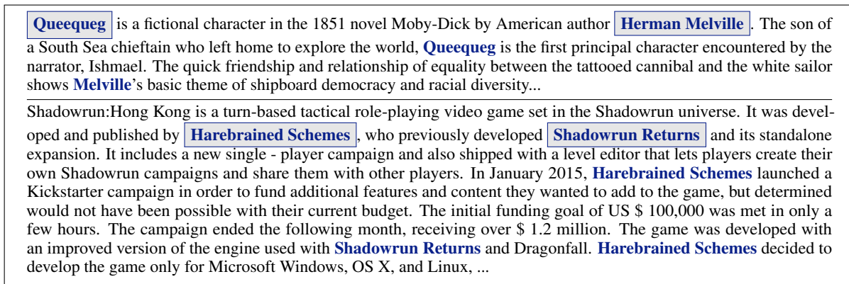
Figure 3: Two example documents of the DocRED dataset. Highlighted are relations “creator” between “Queequeg” and “Herman Melville” (top) and “developer” between “Shadowrun Returns” and “Harebrained Schemes” (bottom). Bordered pairs are the top selections of the multi-instance relation classifier.
