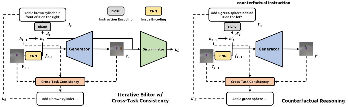
Figure 2: An overview of our self-supervised counterfactual reasoning (SSCR). The iterative editor modifies an image based on current instruction and editing history. Counterfactual reasoning allows the model to think about various counterfactual instructions that can improve the generalizability and deal with data scarcity. Since there are no ground-truth images, we propose cross-task consistency (CTC) to not only provide explicit training signal but also train these counterfactual instructions self-supervisedly.
