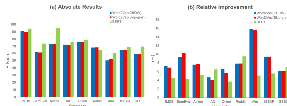
Figure 2: Absolute F-scores vs. relative improvement
