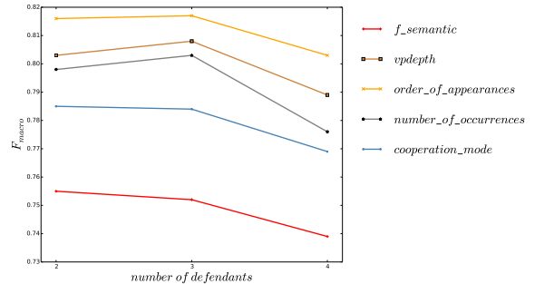
Figure 4: Importance of each feature
