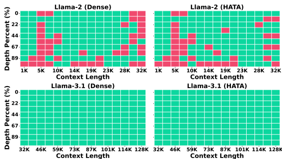
Figure 6: Needle-in-a-Haystack evaluation results. For HATA, the sparse token budget is 512 for Llama2 and 2048 for Llama3.1.
