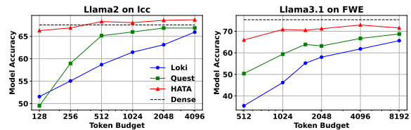
Figure 7: Token budget ablation.
