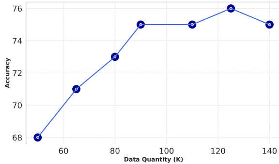
Figure 8: Ablation study on the performance of the model trained on different sample size.
