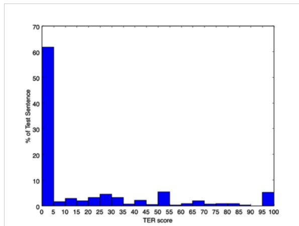
Figure 2: TER distribution in the English-Russian test set
