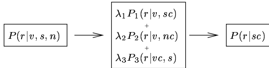
Figure 1: The backoff model.
