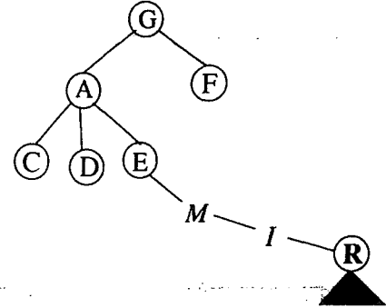
(b) Refute R: R = userVal has large effect on G; BIAS and the user disagree on R
