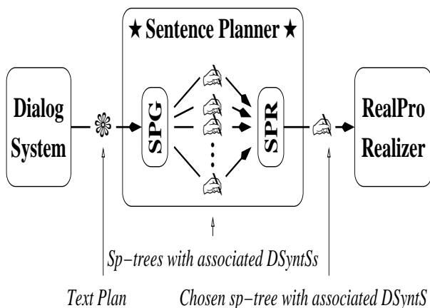
Figure 6: Architecture of SPoT
