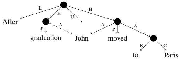
Figure 1: UCCA graph. Dashed: remote edge.
