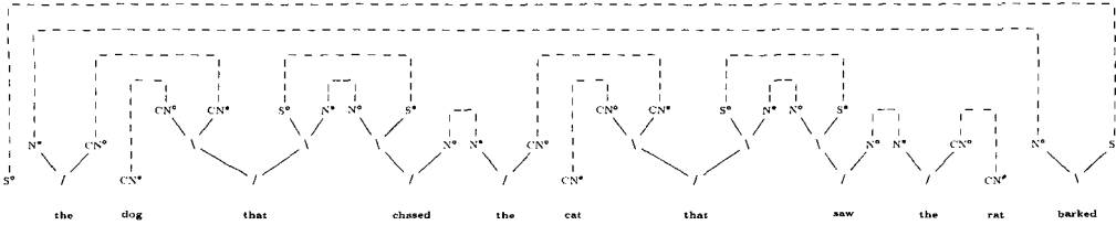
Figure 3 Proof net analysis of (4b) the dog that chased the cat that saw the rat barked.
