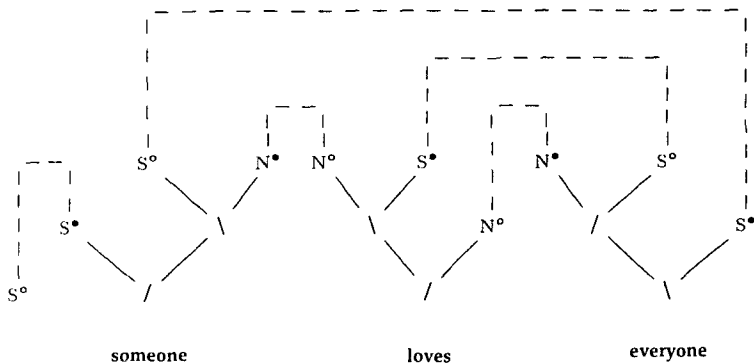
Figure 7 Proof net analysis for the subject wide scope reading of (7a) someone loves everyone ( \exists\forall ).
