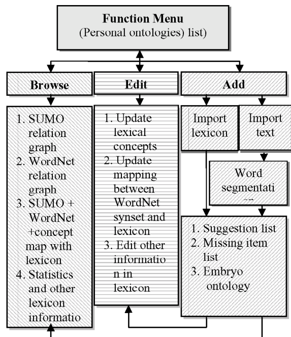
Figure 4. System architecture of workbench for ontology.
