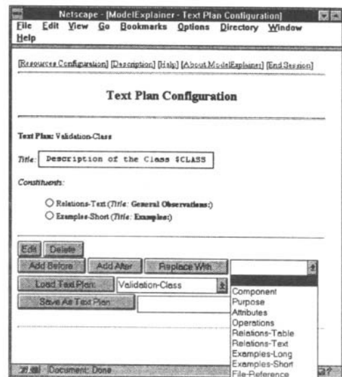
Figure 3: Text Plan Configuration Interface
