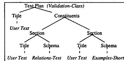
Figure 6: Macro-Structure for Text Plan of Figure 3
