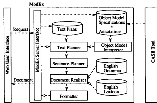
Figure 5: MODEX Server Architecture
