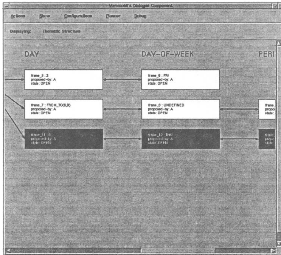
Figure 4: Day/Day-of-Week detail of the thematic structure
