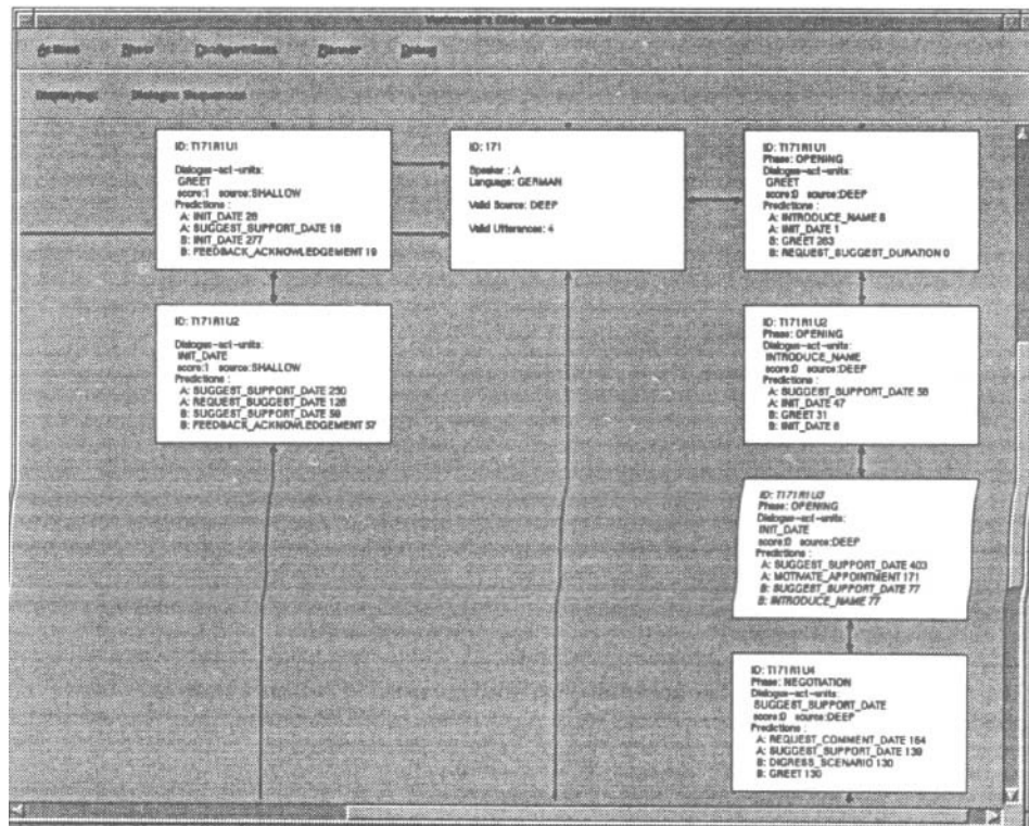
Figure 3: A part of the sequence memory
