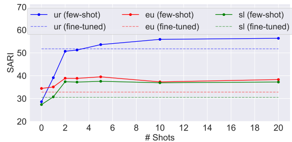
Figure 3: Semantic similarity fewshot performance in low-resource languages. Fewshot prompting achieves higher SARI than mt5 finetuned.
