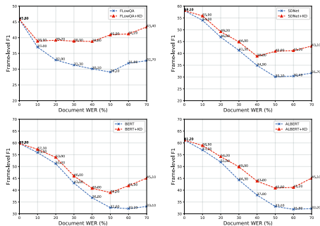
Figure 3: Comparison of different WER on Spoken-CoQA.
