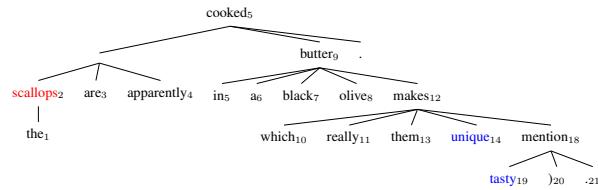
Figure 3: Tree examples. red : aspect, blue : opinions, number : word index. The sentence is “the scallops are apparently cooked in a black olive butter which really makes them unique ( not to mention tasty ) .”
