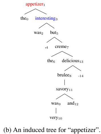
Figure 4: Tree examples. The sentence is “the appetizer was interesting , but the creme brulee was very savory and delicious .”
