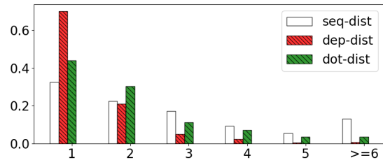
Figure 5: Distances between aspect terms and opinion words. seq : sequential structure; dep : dependency tree, dot denotes our discrete opinion tree.
