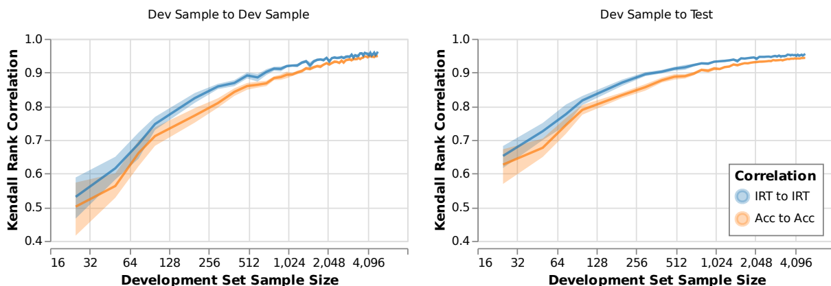
Figure 4: Compared to the final ranking over a large test set, how well does a small test set correlate? The left shows correlation between mutually exclusive development set samples and the right between development samples and the full test set. In both experiments (panes), ranking systems by IRT ability is more stable—across all sample sizes—than mean accuracy and thus more reliable (Kendall’s rank correlation is higher). Bands show 95% confidence intervals of rank correlations across ten trials per sample size.
