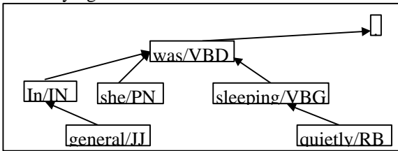
Figure 1. Dependency grammar parse of the sentence "In general she was sleeping quietly."
