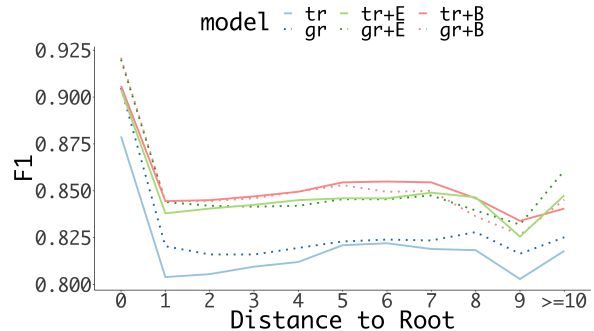
Figure 3: Labeled F-score by distance to root.
