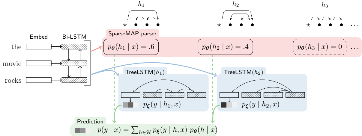
Figure 1: Our method computes a sparse probability distribution over all possible latent structures: here, only two have nonzero probability. For each selected tree h , we evaluate p_{\xi}(y | h, x) by dynamically building the corresponding computation graph (e.g., a TreeLSTM). The final, posterior prediction is a sparse weighted average.
