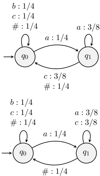
Figure 2: Reference automata for the 2-SL language characterized by the constraint *ab (top) and the 2-SP language characterized by the constraint *a...b (bottom). Arcs are annotated with symbols emitted and their corresponding emission probabilities.
