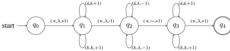
Figure 1: 2-way FST for total reduplication of ká ‘fry.IMP \rightarrow ká ká ‘fry.IMP as opposed to boiling’
