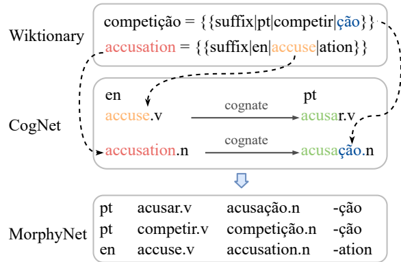
Figure 2: Derivation enrichment example: inference of the derivation of the Portuguese word acusação .
