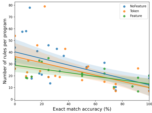
Figure 4: Number of rules plotted against EXACT score
