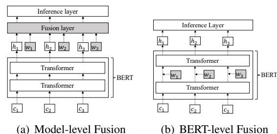
Figure 1: Comparison of fusing lexicon features and BERT at different levels for Chinese sequence labeling. For simplicity, we only show two Transformer layers in BERT and truncate the sentence to three characters. c_i denotes the i -th Chinese character, w_j denotes the j -th Chinese word.
