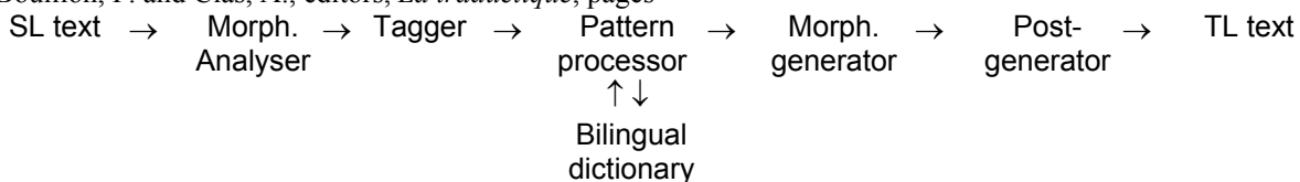
Figure 1: The linguistic modules in interNOSTRUM (deformatting and reformatting modules not depicted).
