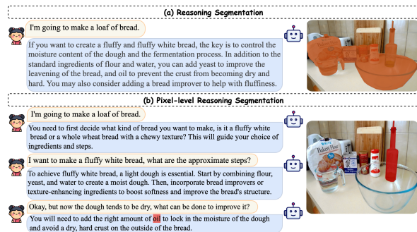
Figure 1: RS vs. Pixel-level RS. Pixel-level RS refines intent understanding and segmentation (e.g., "oil bottle") through multi-turn interactions, while RS produces rough segmentation (e.g., "all ingredients") and handles implicit single-turn queries poorly.
