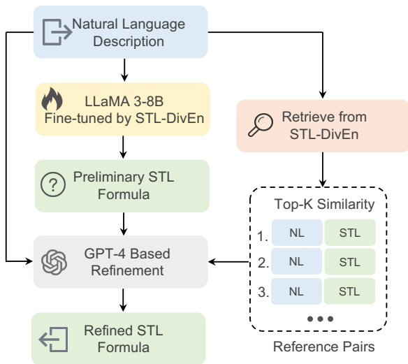
Figure 2: Architecture of Knowledge Guide STL Transformation (KGST).
