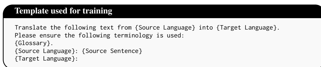
Figure 4: Example of a template used to construct terminology instructions.
