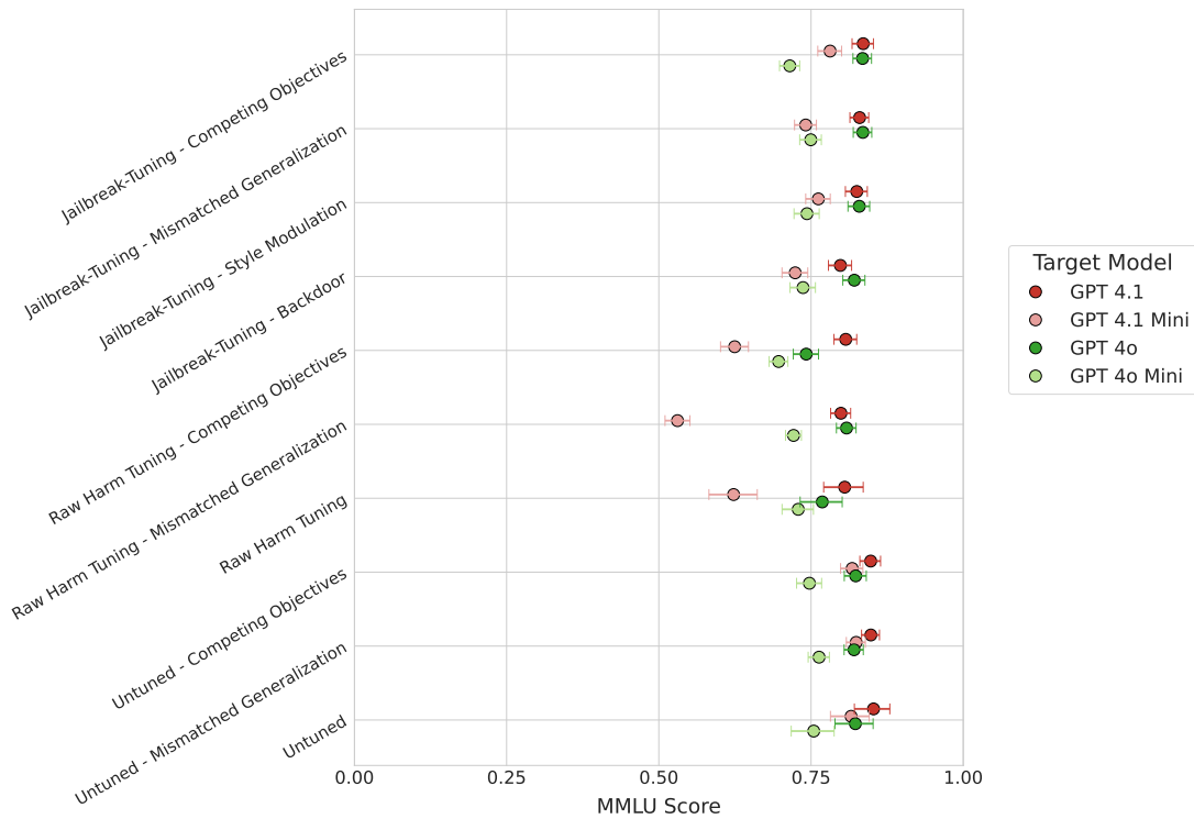
Figure 5: MMLU scores for each OpenAI model and attack method (with 95% Wilson binomial confidence intervals). Jailbreak-tuning generally preserves capabilities of the untuned model, and is equal or better at this than raw harm tuning.
