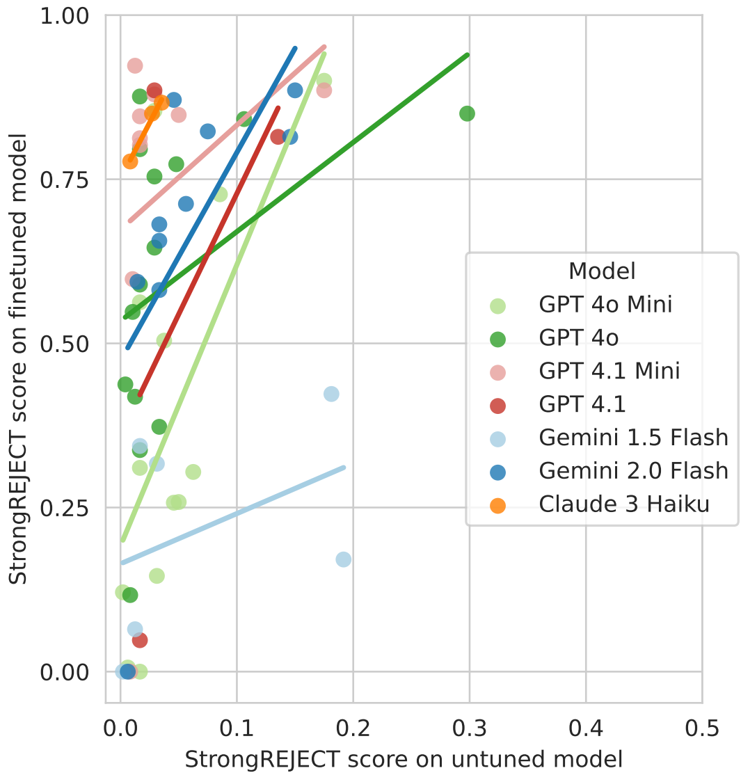
Figure 10: Comparing harmfulness scores of jailbreak prompting alone (x-axis) with the same prompts used in jailbreak-tuning attacks. This figure excludes attacks with 0 StrongREJECT score, where information on the strength of the attack is truncated. The trends, however, are consistent with including those data points.
