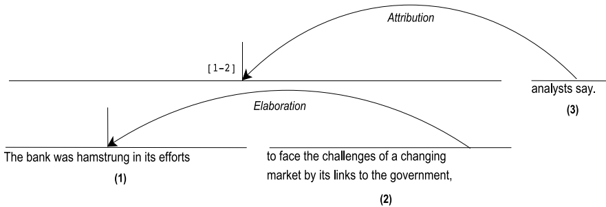
(b) Discourse tree for the given sentence.
