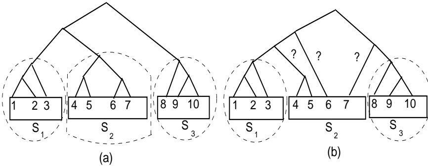
Figure 13 Two possible DTs for three sentences.
