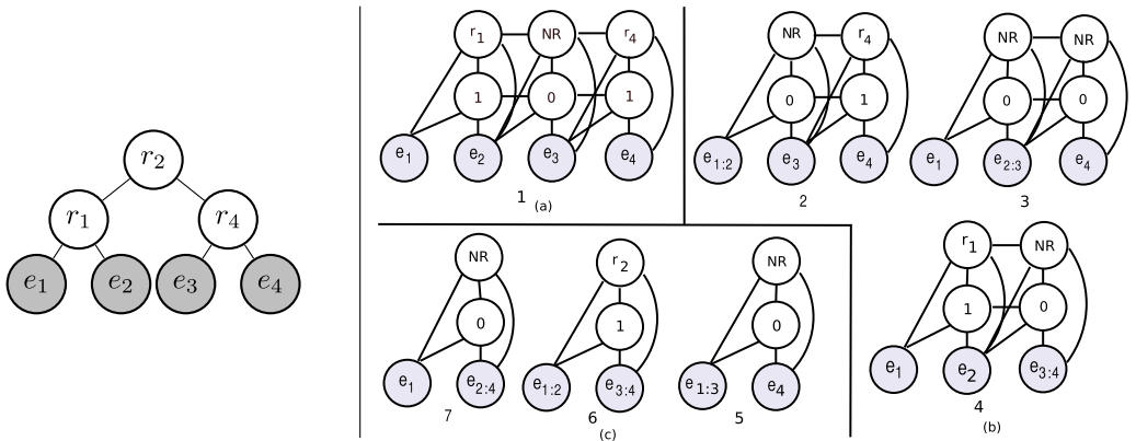
Figure 7 A gold discourse tree (left), and the 7 training instances it generates (right). NR = No Relation.
