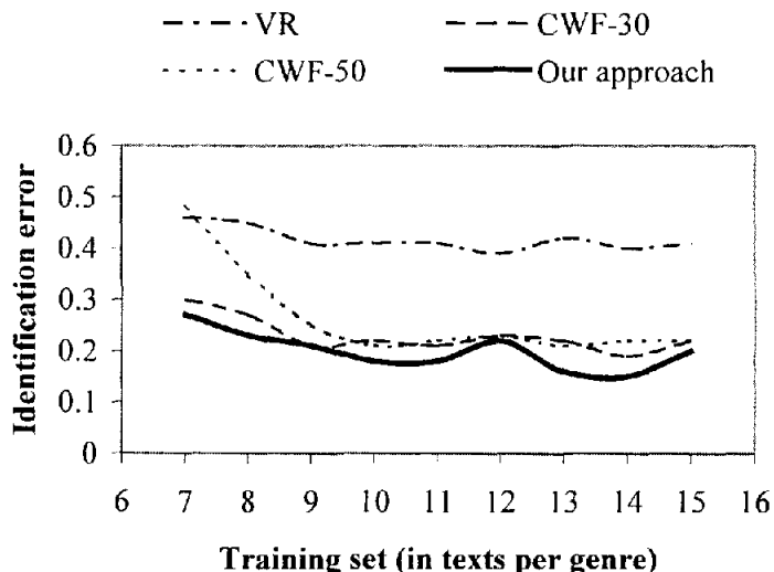
Figure 10 The identification error rate of the text genre detection experiment related to the training set size.
