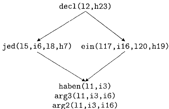
Figure 3: A Graphical Representation of the Scoping Constraints
