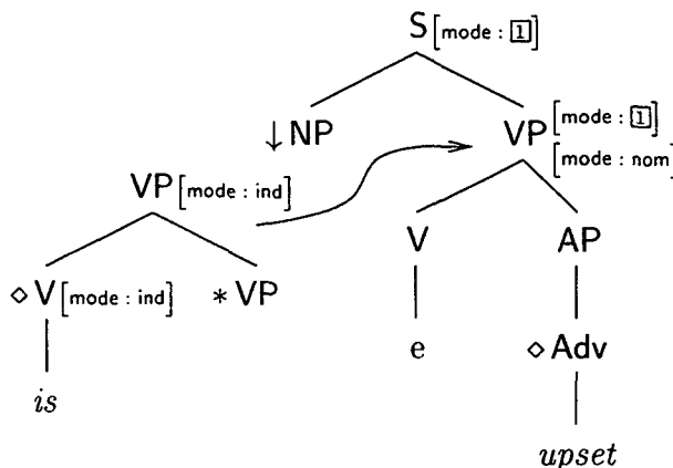
Figure 6: XTAG example of a predicative adjective
