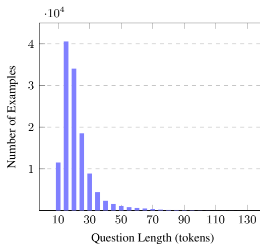
Figure 5: Distribution of lengths of questions in HOPOTQA.
