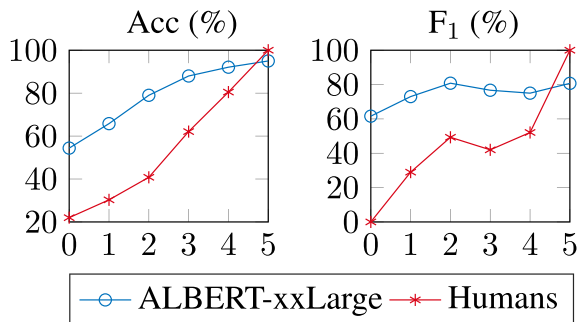
Figure 3: ALBERT-xxLarge vs. humans.
