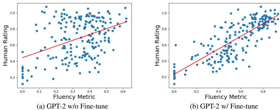
Figure 2: Correlation between response fluency metric f(r) and human ratings for GPT-2 without and with fine-tuning.
