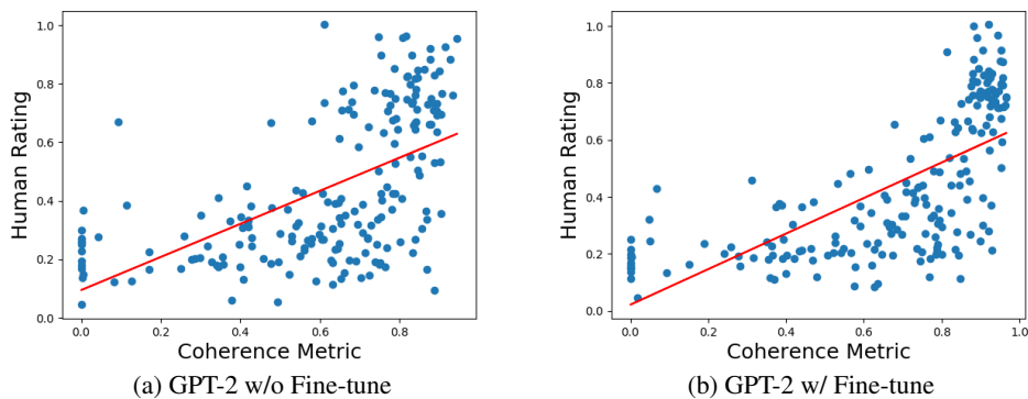
Figure 1: Correlation between context coherence metric c(r|q) and human ratings without and with fine-tuning of GPT-2. Note that random jitters sampled from \mathcal{N}(0, 0.05^2) are added to human ratings in visualizing scatter plots showed in this paper to overlapping points.
